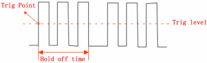
Figure 2-36 Trigger hold-off schematic figure
