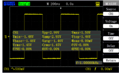
Figure 2-56 All measurement
