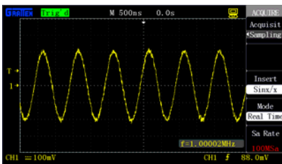
Figure 2-40 Sampling mode
